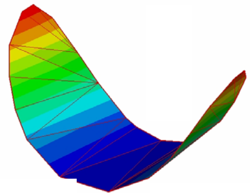
Fig 15: Measured distorted shape of Pressure Bulkhead
